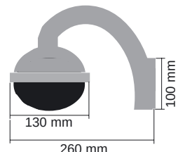
with wall mount for outdoor
