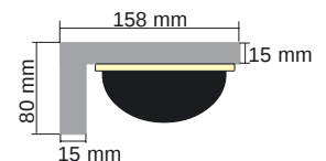
with wall mount for indoor
