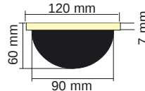
with ceiling mount for outdoor
