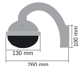
with wall mount for outdoor
