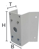
Art.no. 20616 Corner assembly mount for wall mount Measurements: B= 195mm H= 220mm T= 120mm
